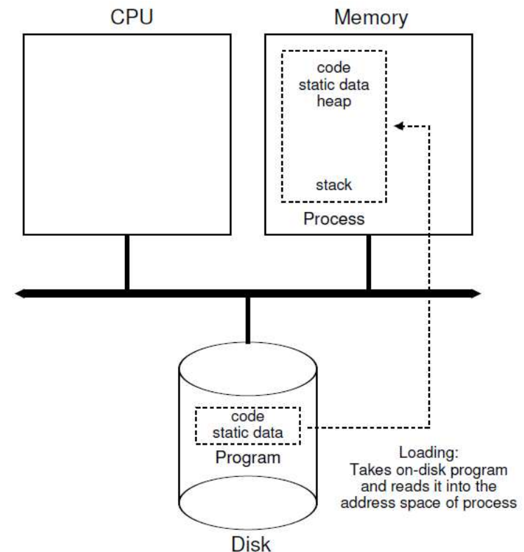
Figure 4.1: Loading: From Program To Process
