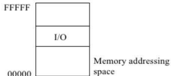
Memory-mapped I/O
