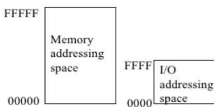
Direct I/O
