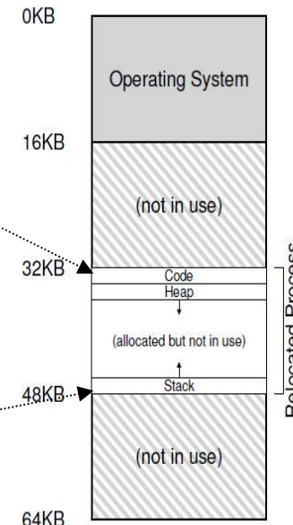
Figure 15.2: Physical Memory with a Single Relocated Process_hoi, DKU
