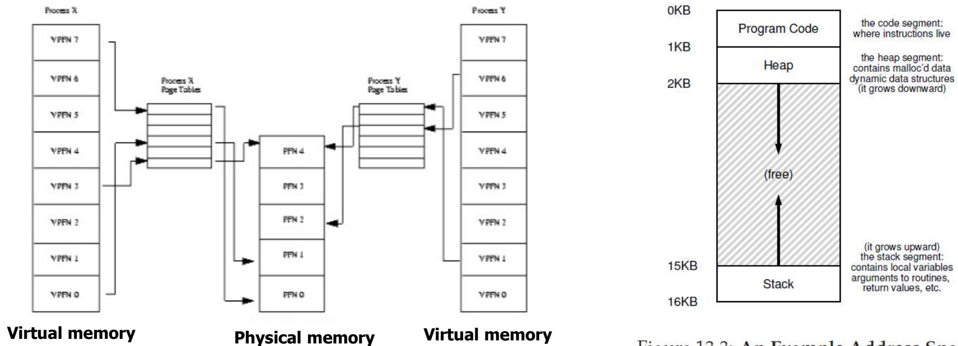
Figure 13.3: An Example Address Space
