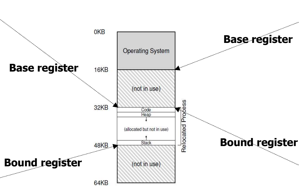
Figure 15.2: Physical Memory with a Single Relocated Process
