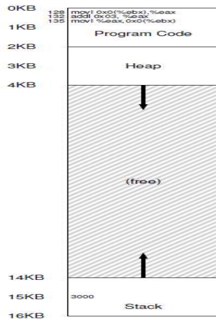
Figure 15.1: A Process And Its Address Space
