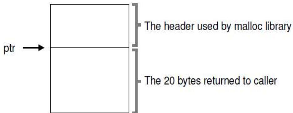
Figure 17.1: An Allocated Region Plus Header
