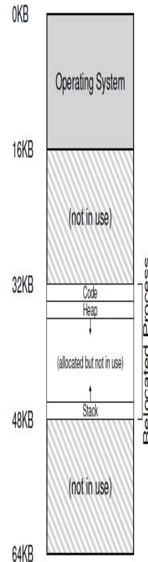
Figure 15.2: Physical Memory with a Single Relocated Process
