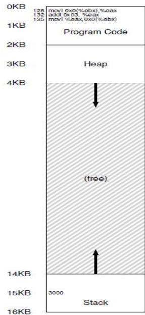
Figure 15.1: A Process And Its Address Space
