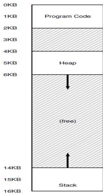
Figure 16.1: An Address Space (Again)
