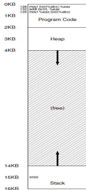
Figure 15.1: A Process And Its Address Space
