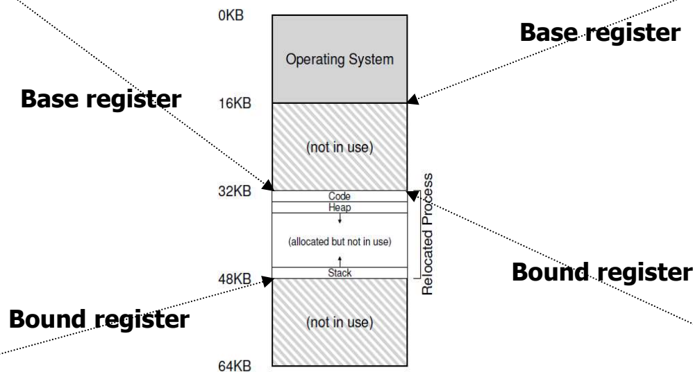
Figure 15.2: Physical Memory with a Single Relocated Process
