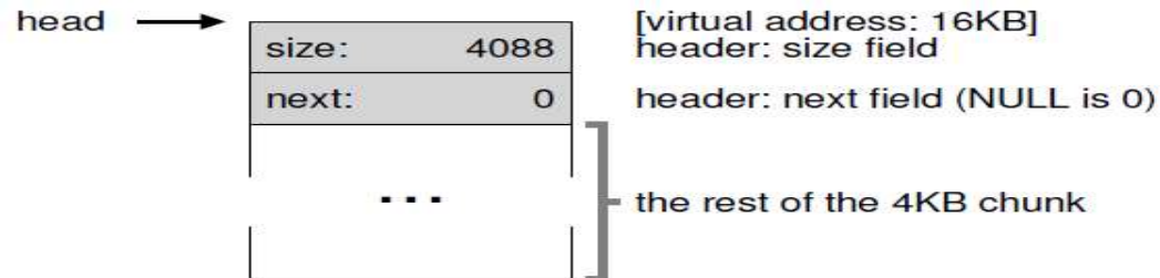
Figure 17.3: A Heap With One Free Chunk
